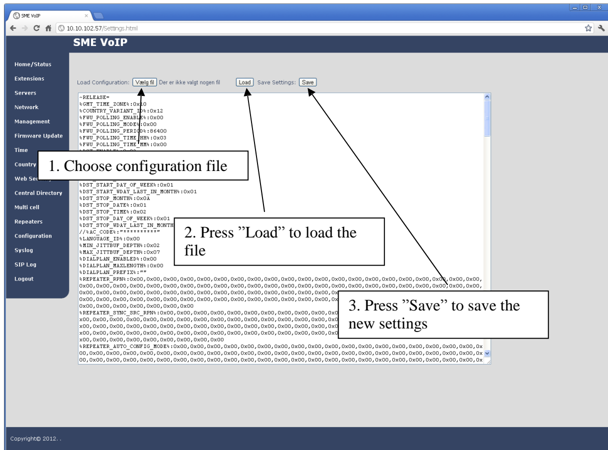
Figure 2. Configuration page.
